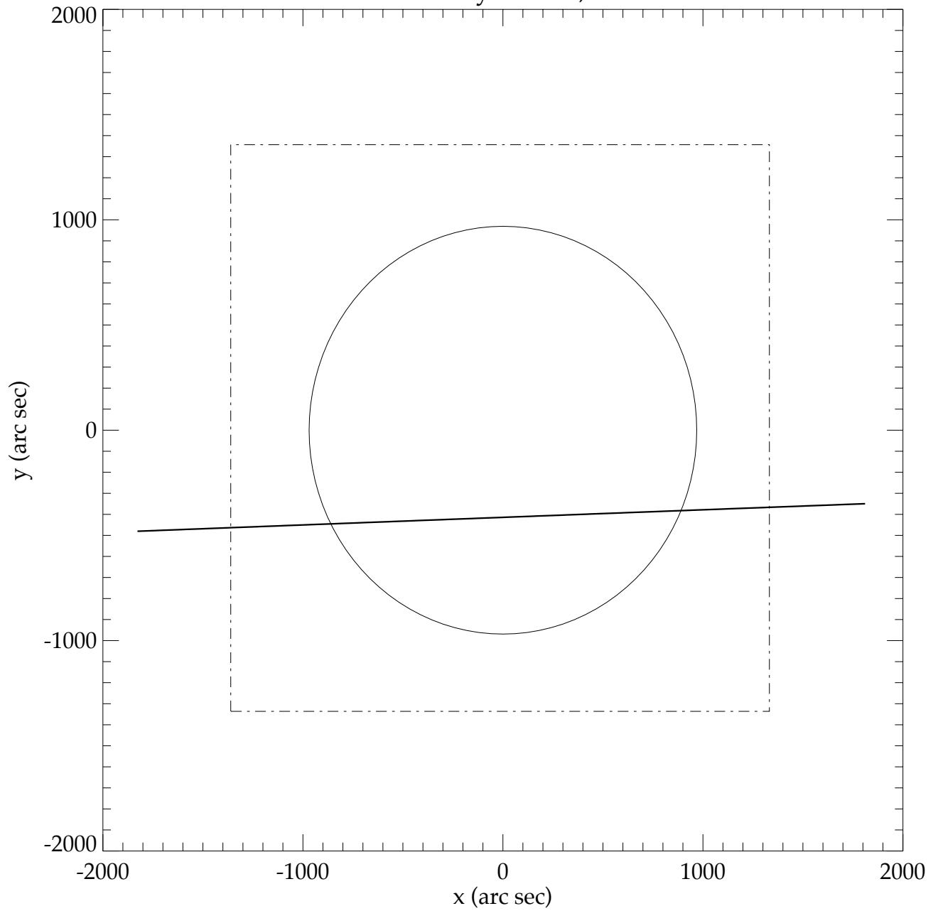
SOHO view of Mercury transit, 2006 November 8
