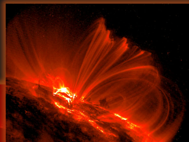
Magnetic loops above active region in extreme UV light (Credit: TRACE)
