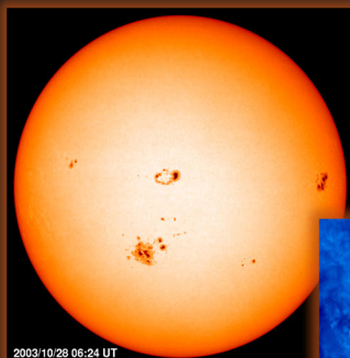
2003/10/28 06:24 UT Sunspots observed in visible light (Credit: SOHO)
