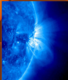
Magnetic loops above active region in UV light (Credit: STEREO)
