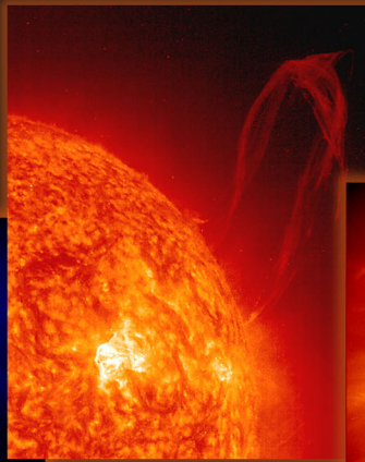
Eruptive prominence in extreme UV light (Credit: SOHO)
